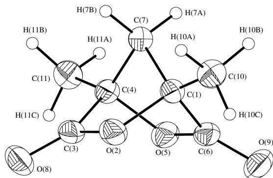
Figure 1 Molecular structure of dilactone 1 . Atoms C(4), O(5), C(6), O(9), and C(11) are symmetrically equivalent to atoms C(1), O(2), C(3), O(8), and C(10), respectively. Selected bond lengths (Å): C(1)–O(2) 1.491(3), C(1)–C(6) 1.536(3), C(1)–C(7) 1.530(3), C(1)–C(10) 1.490(3), O(2)–C(3) 1.366(3), C(3)–O(8) 1.193(2); selected bond and dihedral angles (°): C(1)–O(2)–C(3) 106.3(1), C(1)–C(6)–O(5) 106.3(2), C(1)–C(7)–C(4) 92.8(2), O(2)–C(1)–C(6) 102.6(2), O(2)–C(1)–C(7) 101.7(2), O(2)–C(1)–C(10) 110.0(2), C(6)–C(1)–C(7) 99.3(2), C(6)–C(1)–C(10) 117.5(2), C(7)–C(1)–C(10) 123.0(2), O(2)–C(3)–O(8) 123.2(2), C(4)–C(3)–O(8) 130.4(2), C(1)–O(2)–C(3)–C(4) ( \tau_0 ) 1.8, C(1)–O(2)–C(3)–O(8) –179.8.
