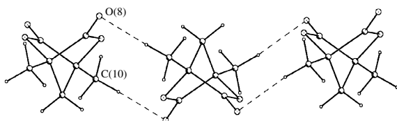
Figure 2 Hydrogen-bonded heterochiral chain in the crystal structure of 1 . Geometry parameters of short C(10)–H(10B)⋯O(8) contacts: H⋯O 2.40 Å, C⋯O 3.393(3) Å, C–H⋯O 155°, H⋯O=C 122.7°.
